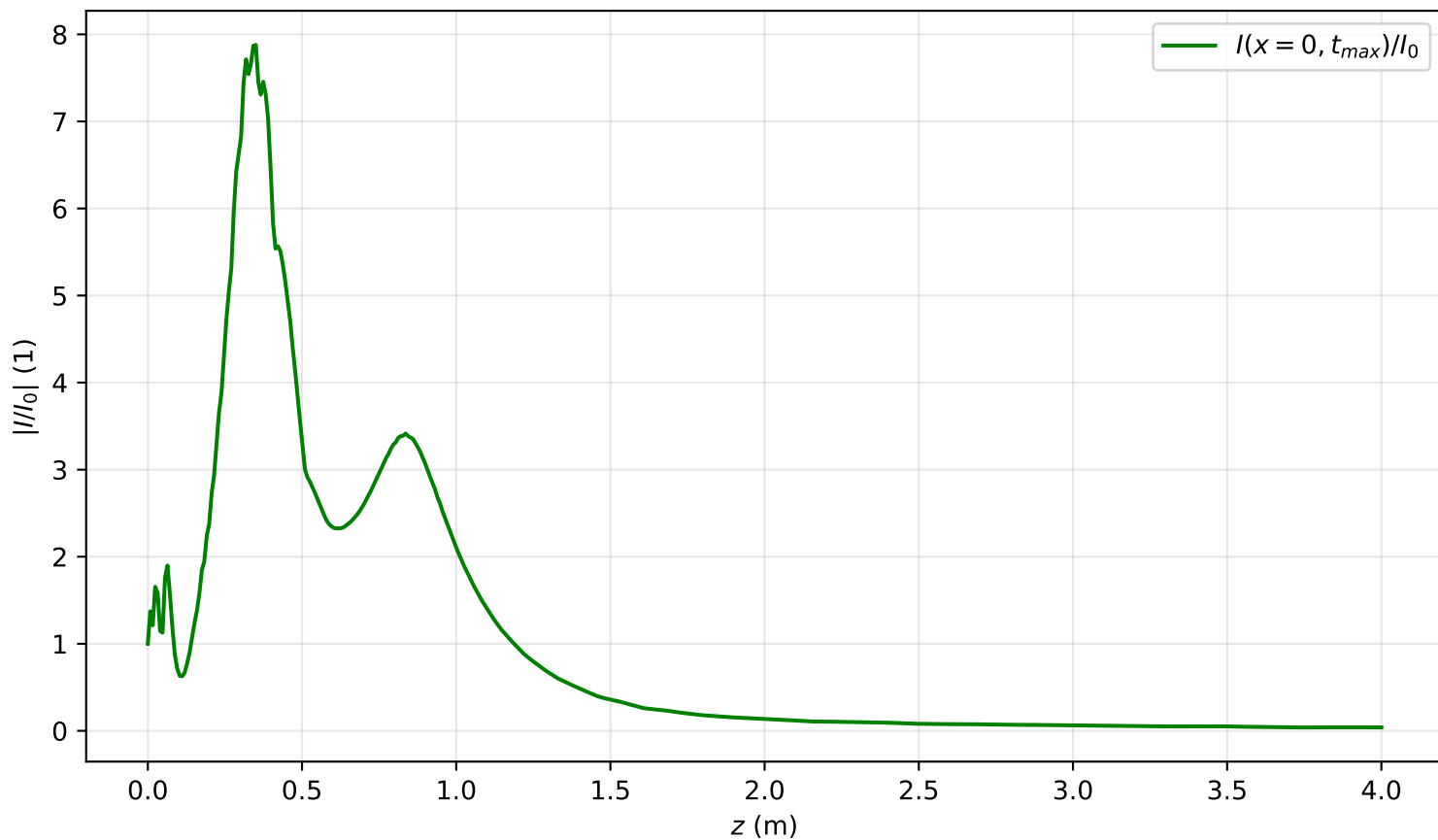
I(x=0, t_{max}, z)/I_0 , Pin=4.4Pcr
